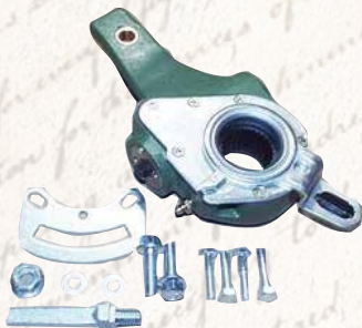
HALDEX STYLE SLACK ADJUSTER 5.5 OR 6" CENTER
